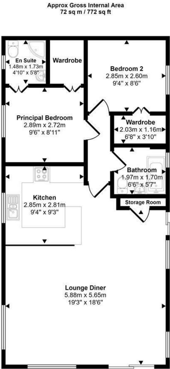
Floorplan
